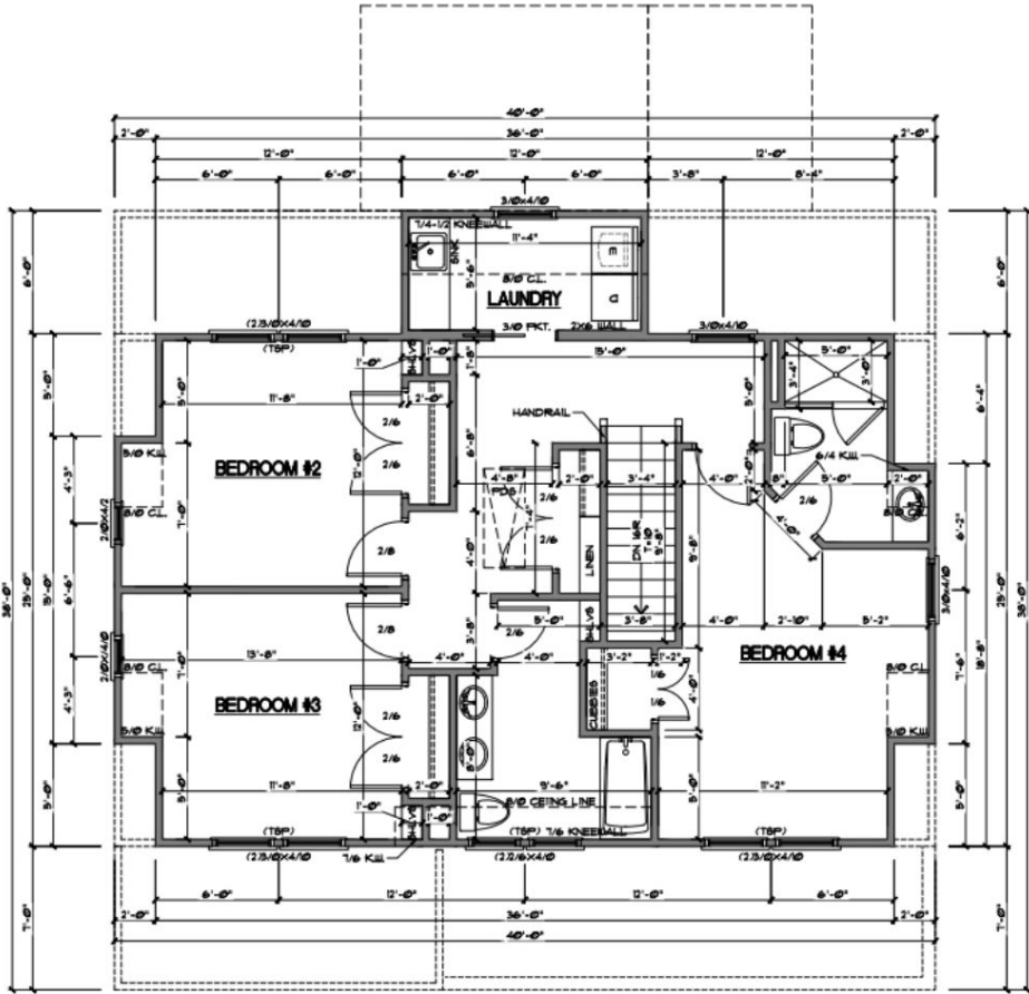
SECOND FLOOR SCALE: 1/8"=1'
