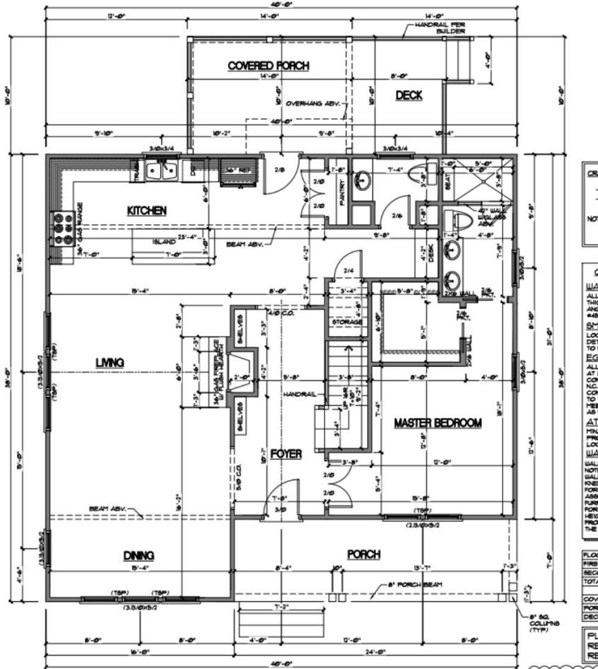
FIRST FLOOR SCALE : 1/8"=1'
